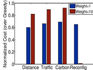
Fig. 12: Reconfiguration
