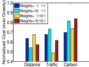
Fig. 11: Tuning Weights
