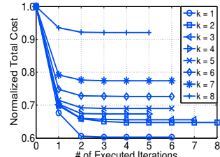
Fig. 13: Convergence
