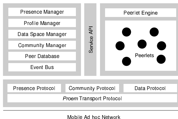
Figure 3. Runtime Architecture
