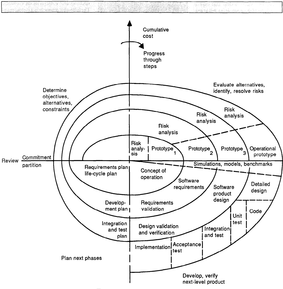
Figure 2. Spiral model of the software process.
