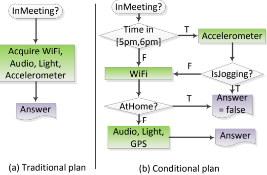
Figure 7: A conditional acquisition plan that acquires different sensor data depending on various conditions
