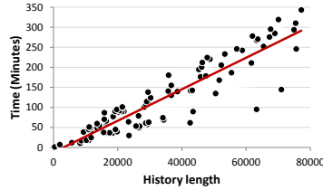
Figure 4: Time required to learn rules on a Samsung Focus phone
