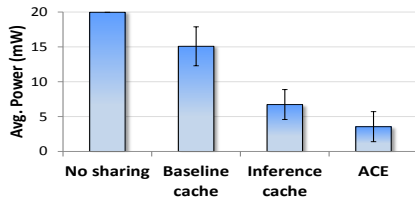
Figure 14: End-to-end energy savings
