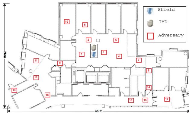
Figure 6—Testbed setup showing shield, IMD, and adversary locations. We experiment with 18 adversary locations, numbered here in descending order of received signal strength at the shield.
