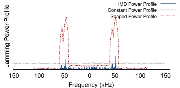
Figure 5 —Shaping the jamming signal’s profile to match an IMD’s allows the shield to focus its jamming power on the frequencies that matter for decoding, as opposed to jamming across the entire 300 KHz channel.
