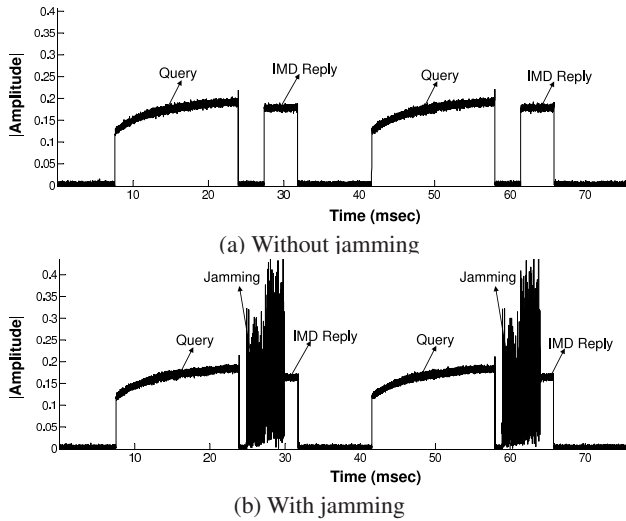
Figure 3 —Typical interaction between the Virtuoso IMD and its programmer: Without jamming (a), the IMD transmits in response to an interrogation. The bottom graph (b) shows that the IMD transmits within a fixed interval without sensing the medium.
