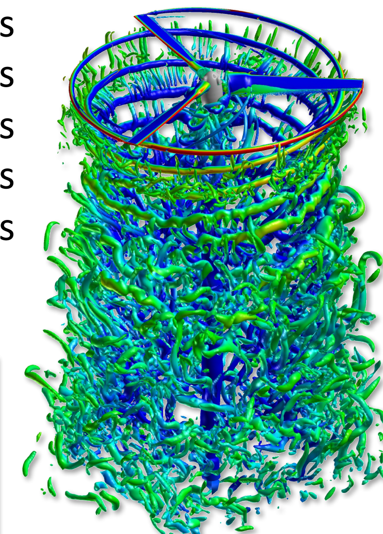
Coupled Helios-FUN3D Simulation Courtesy Rohit Jain, US Army Aviation Development Directorate - AFDD
