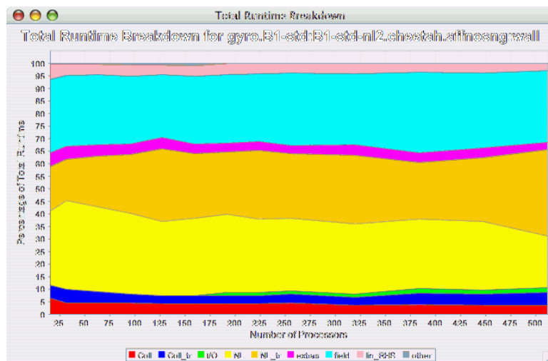
Figure 24.13. Runtime Breakdown
