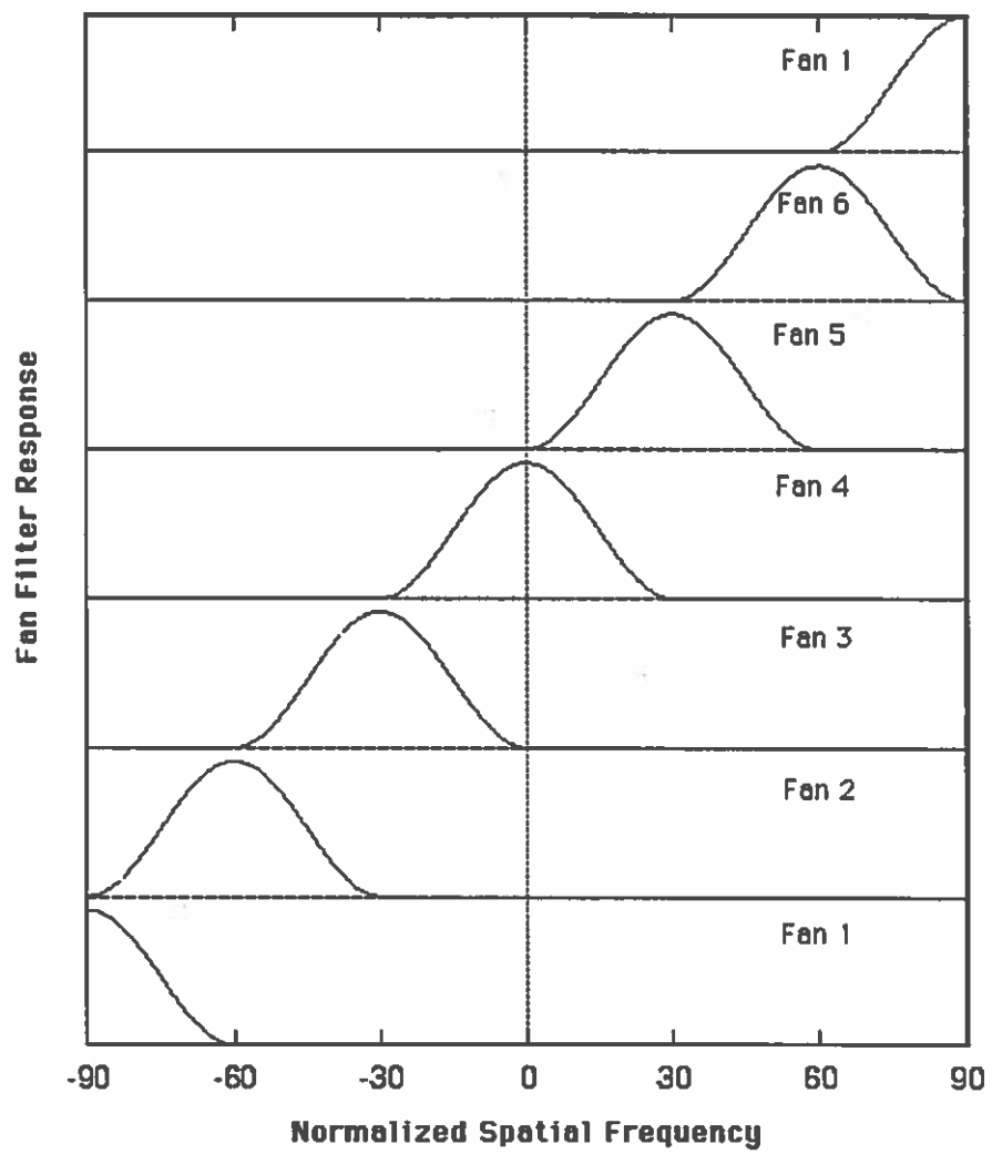
FIGURE 10. Fan Filters
