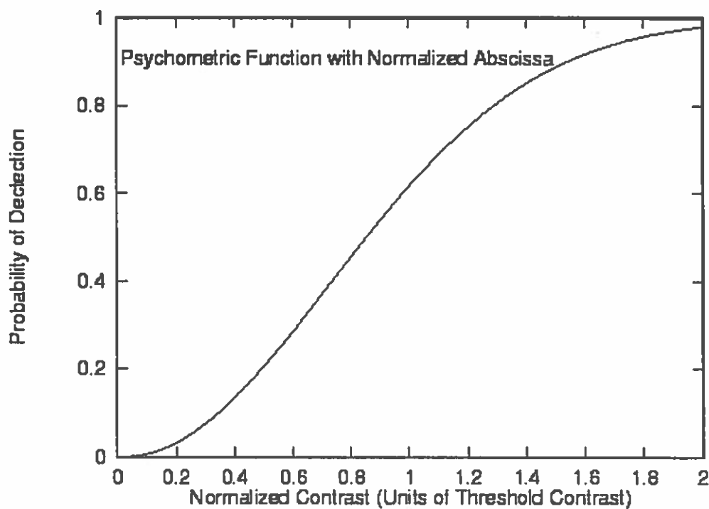
FIGURE 15. Psychometric Function
