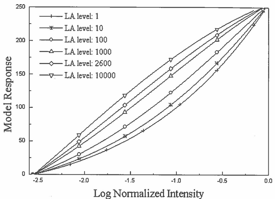
FIGURE 6. Amplitude Nonlinearity
