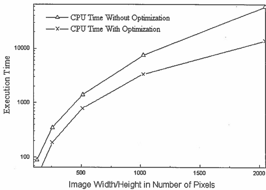
FIGURE 30. Complexity of the Daly Model
