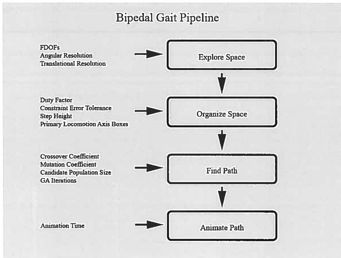
Figure 45. Bipedal gait pipeline.
