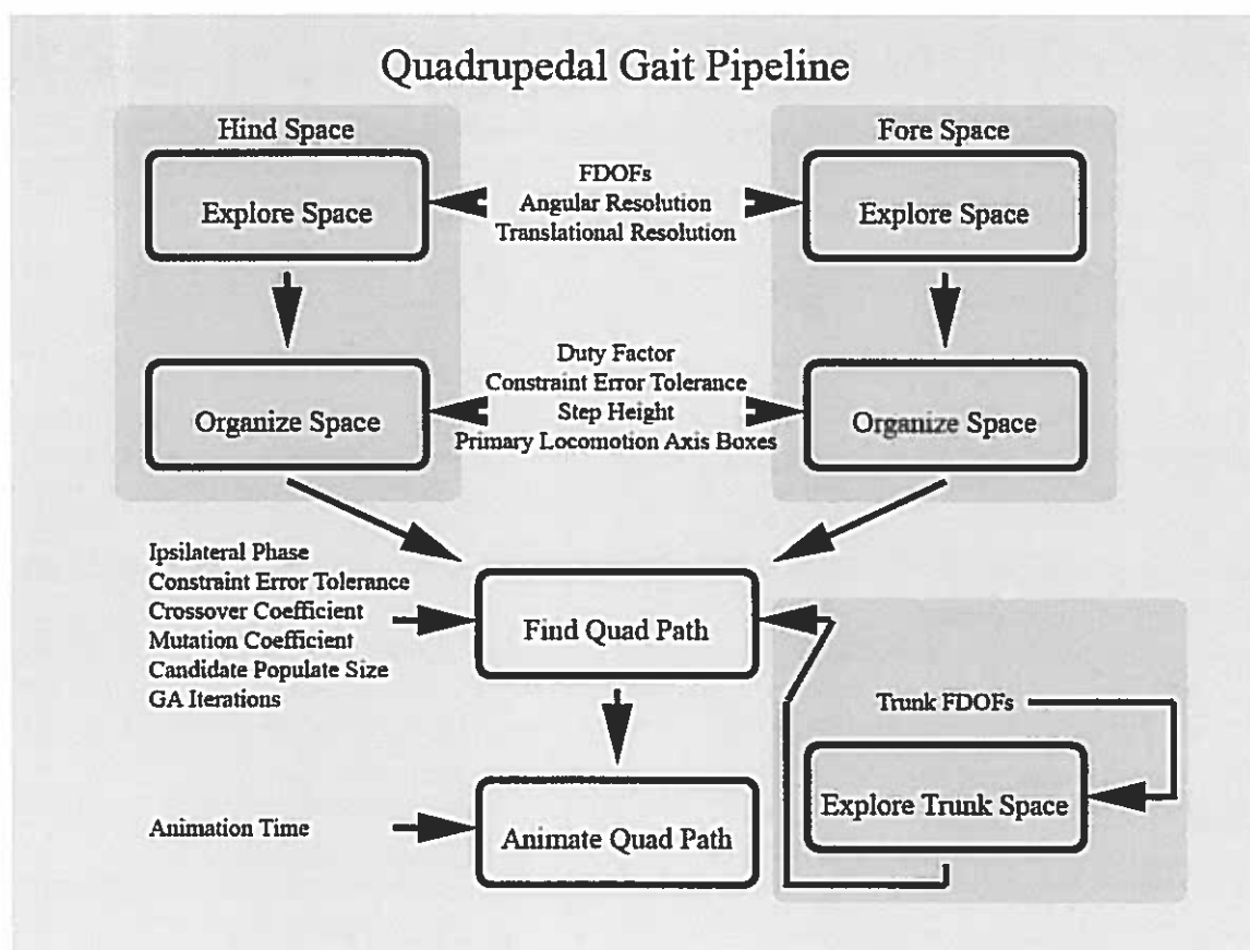
Figure 50. Quadrupedal gait pipeline.
