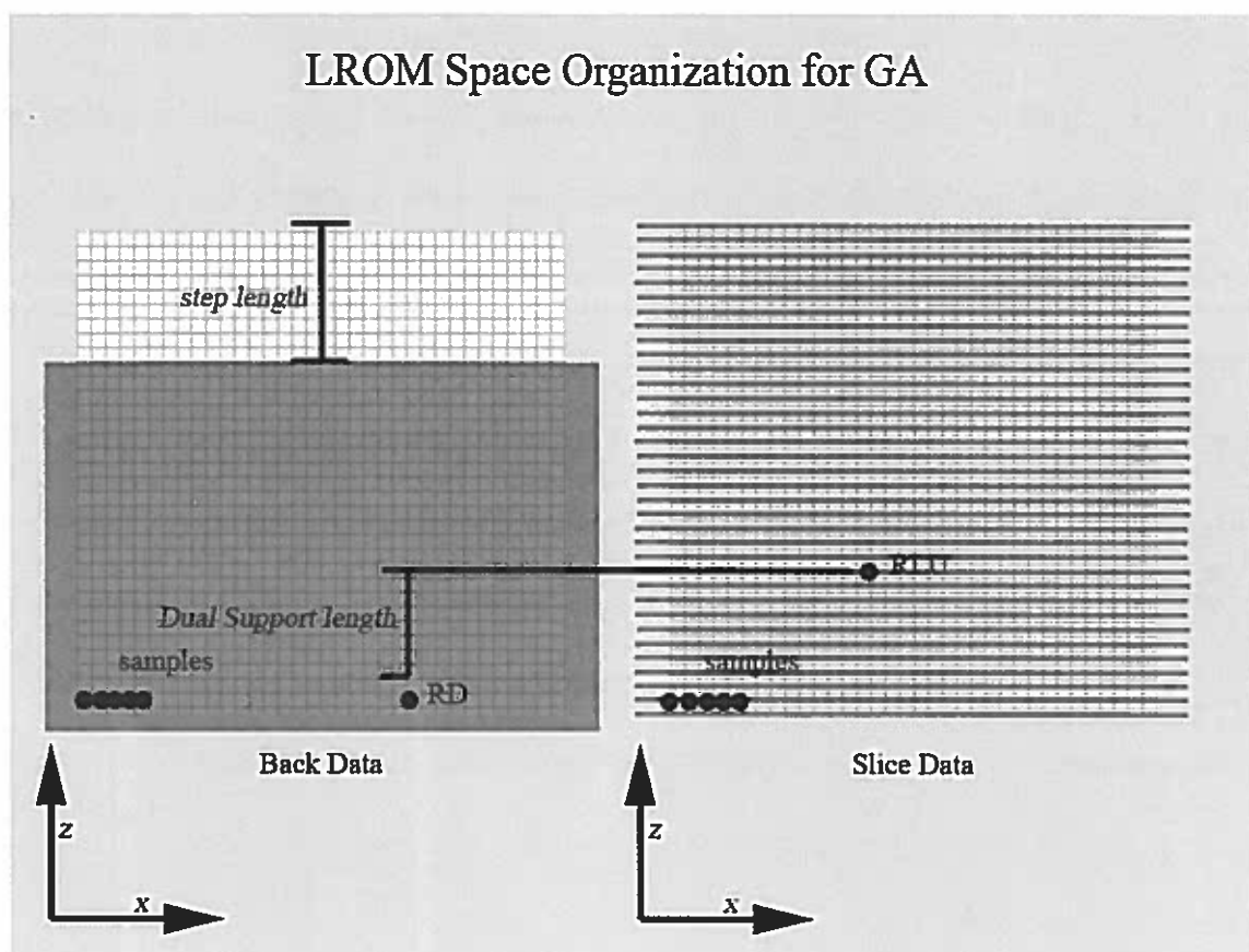
Figure 43. Back data and slice data organization.
