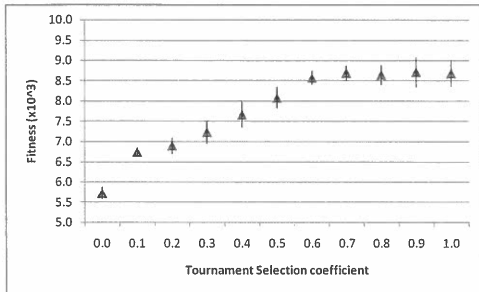
Figure 84. Effect of varying Tournament Selection coefficient.
