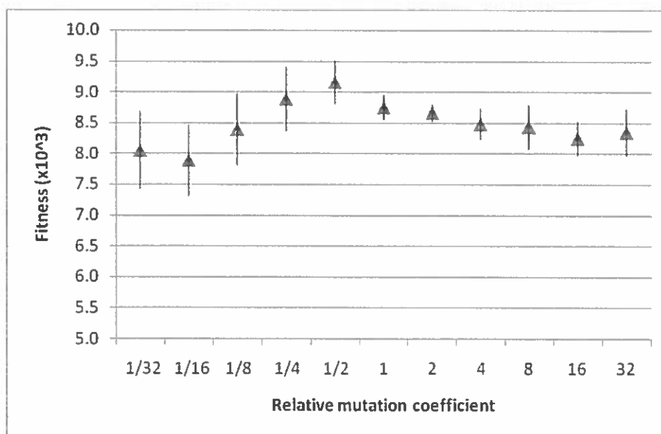
Figure 87. Effect of varying relative mutation coefficient with no crossover.
