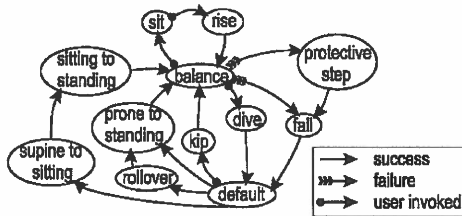
Figure 8. Controller graph.
