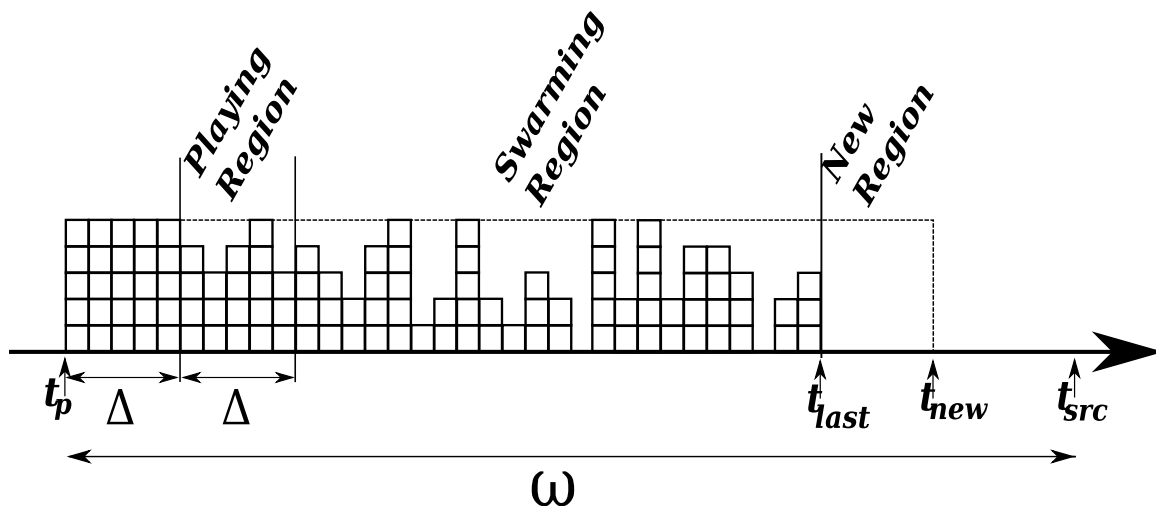
FIGURE 35.: Buffer state at a scheduling event in a peer.
