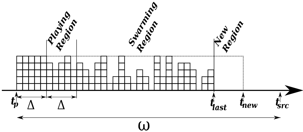
FIGURE 2.: Buffer state at a scheduling event in a peer.
