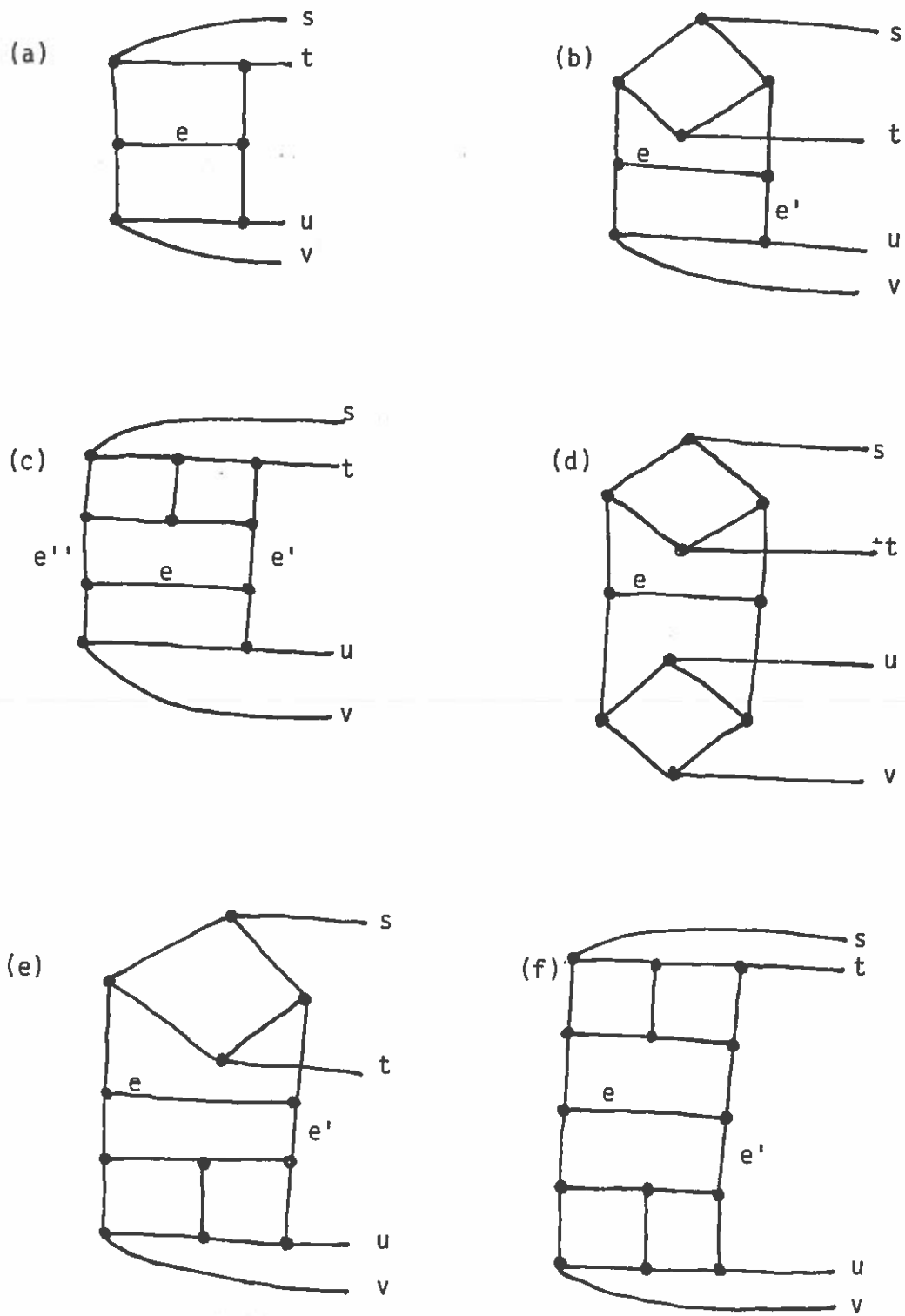
Figure 3: The six cases of an edge neighborhood in a cubic minimal forbidden minor.
