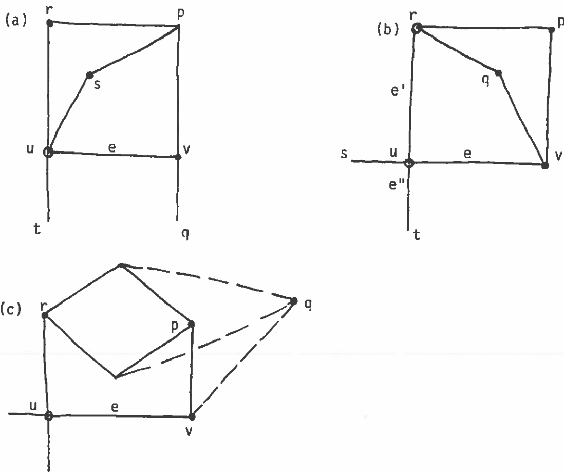
Figure 5: Overlapping cycles in a purported minimal forbidden minor with mixed degree edges; vertices are coded as: \circ degree 4, \bullet degree 3.
