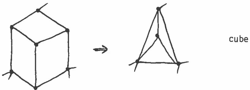
Figure 2: (a) Rewriting rules for recognition of partial 2-trees; (b) rules for the safe reduction of degree 3 vertices in partial 3-trees.
