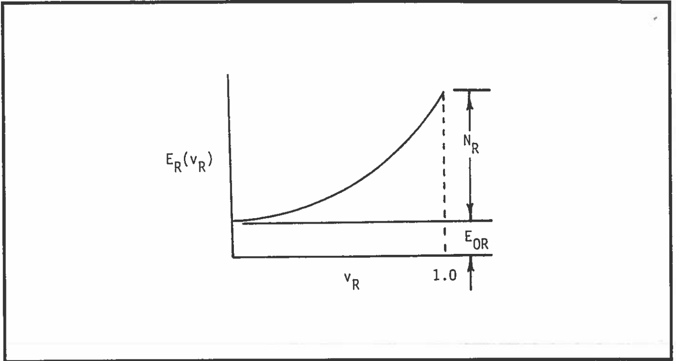
Figure 5: Phosphor excitation function which produces a residual amount of light when the v_R = 0
