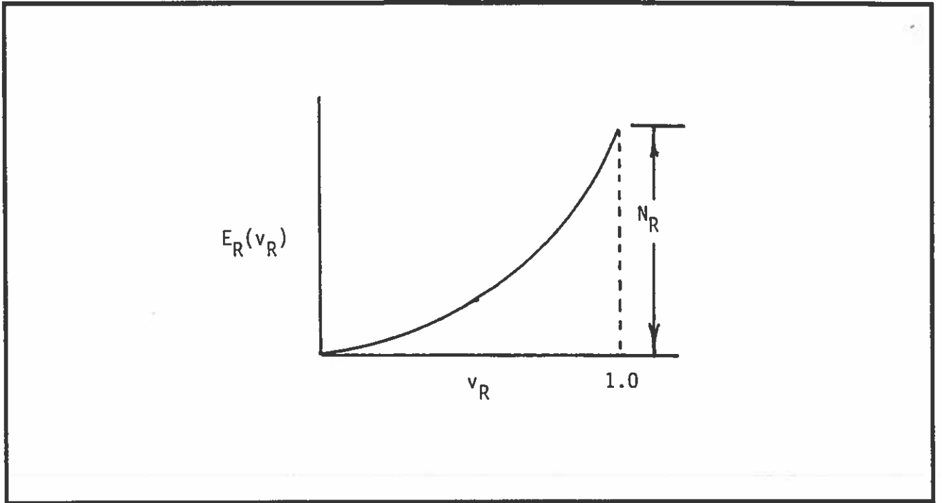
Figure 3: A typical phosphor excitation function
