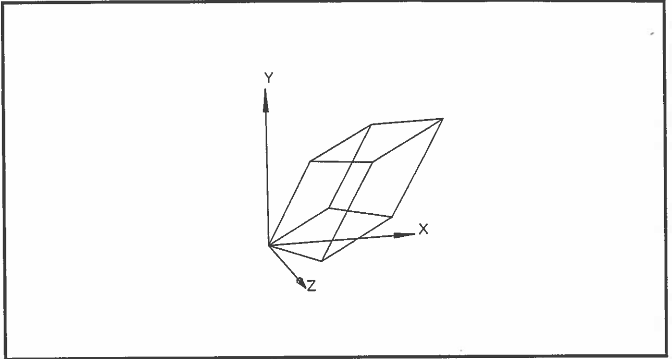
Figure 2: Monitor gamut in CIE XYZ space
