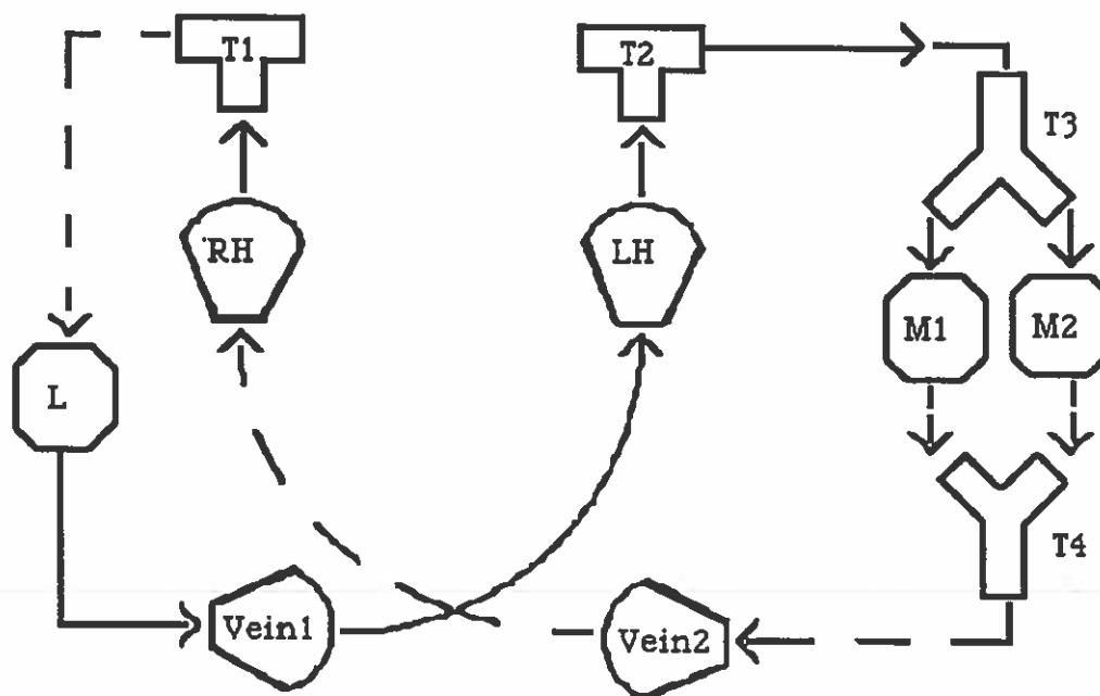
FIGURE 10. The serial crocodilian topology.
