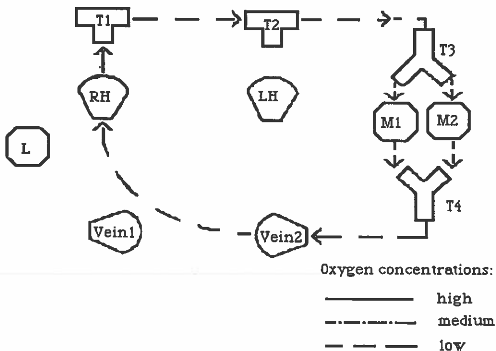
FIGURE 9. The incomplete crocodilian topology.
