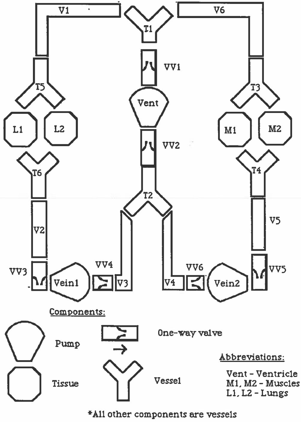
FIGURE 16. Reptilian circulatory model.
