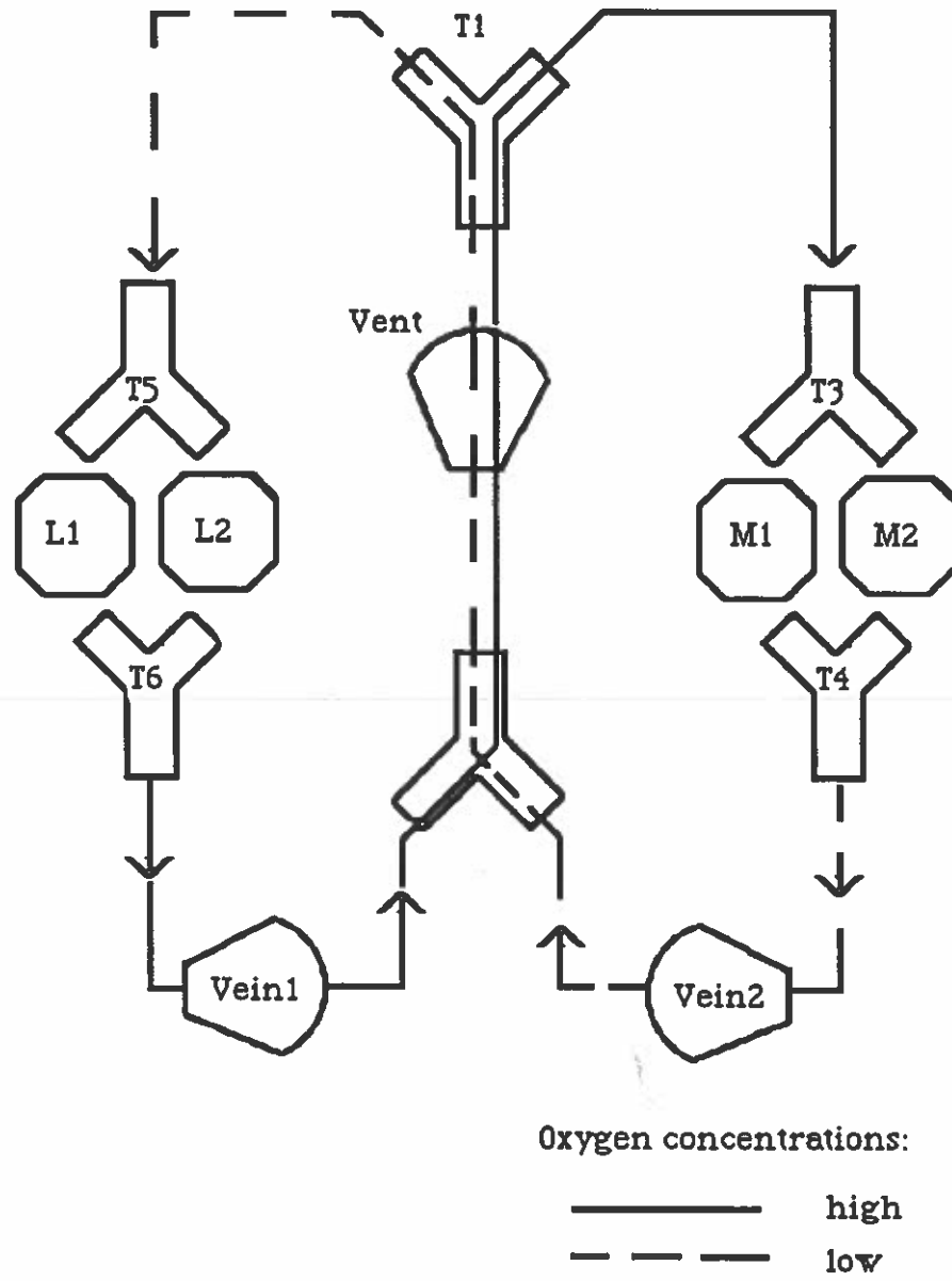
FIGURE 43. The serial reptilian topology.
