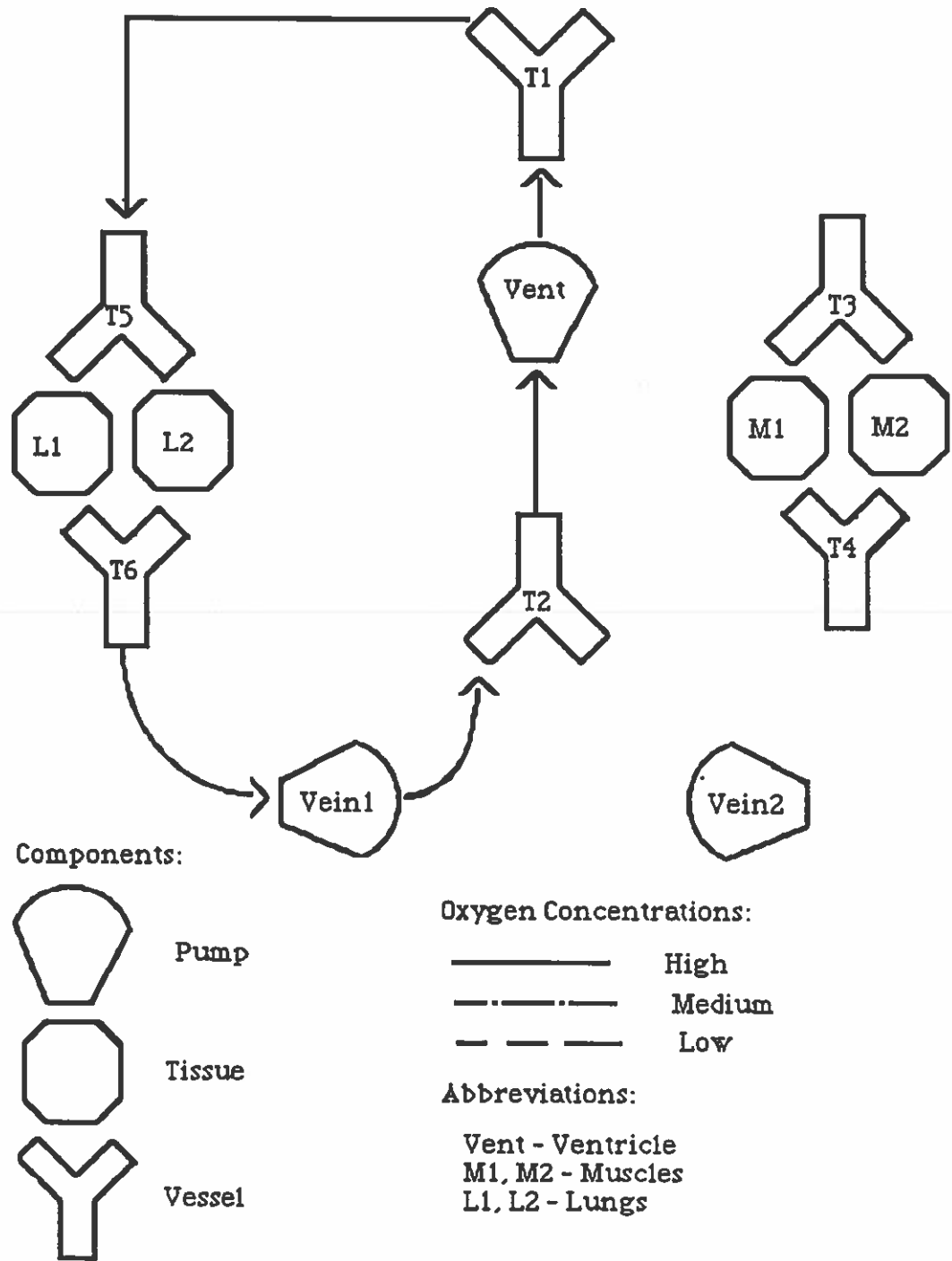
FIGURE 20. Pulmonary reptilian DFN.
