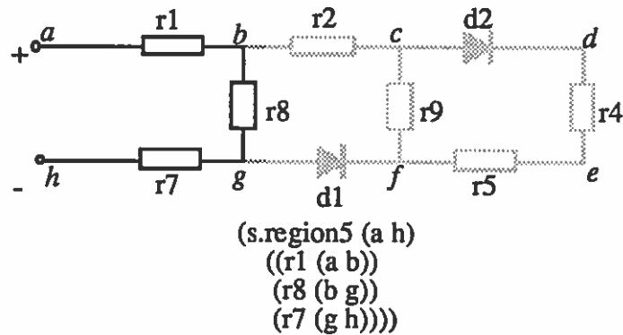
FIGURE 24. Representation of Active Configuration as Regions
