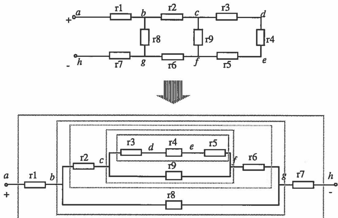
FIGURE 18. Hierarchical View of Ladder Circuit by Clustering
