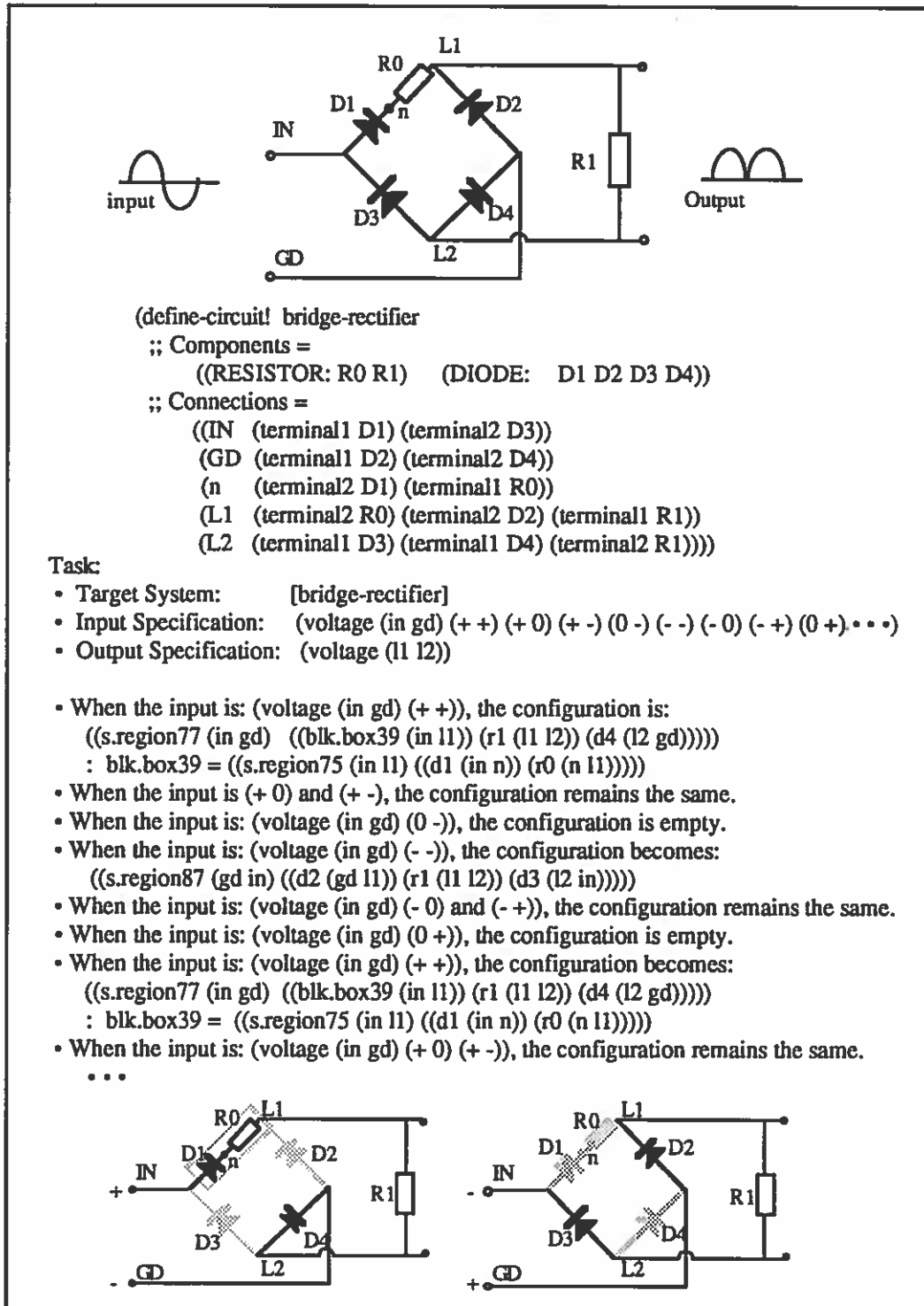
FIGURE 52. Configurations of Full-Wave Bridge Rectifier
