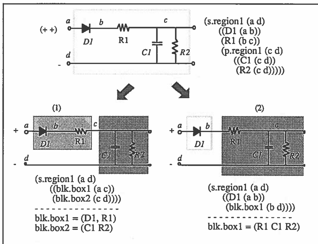
FIGURE 36. Shifting Perspective in the Dimension of Structural Aggregation
