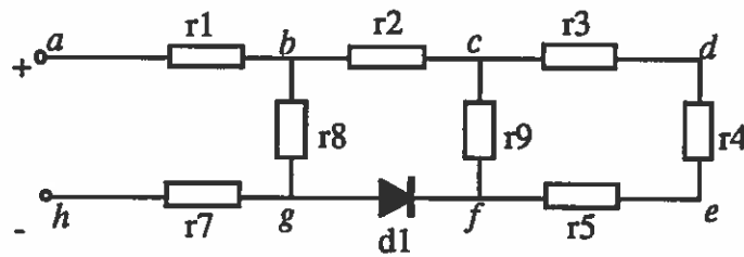
FIGURE 20. Ladder Circuit with Orientation
