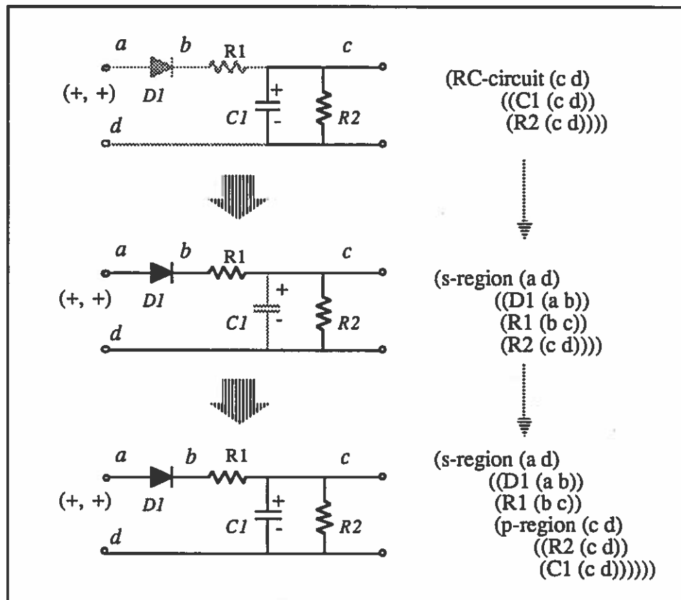
FIGURE 27. Shifting Perspective in the Dimension of Topological Configuration
