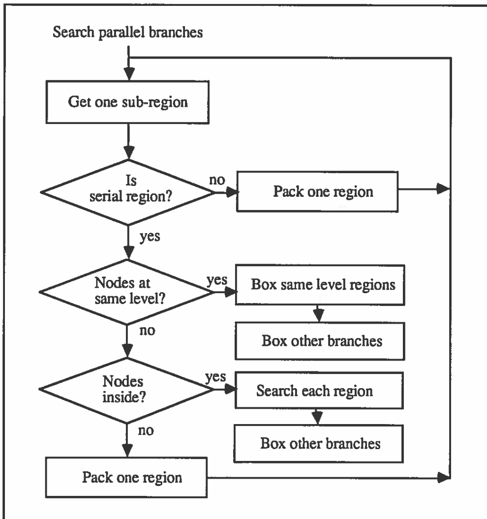
FIGURE 34. Black Boxing in Parallel Region
