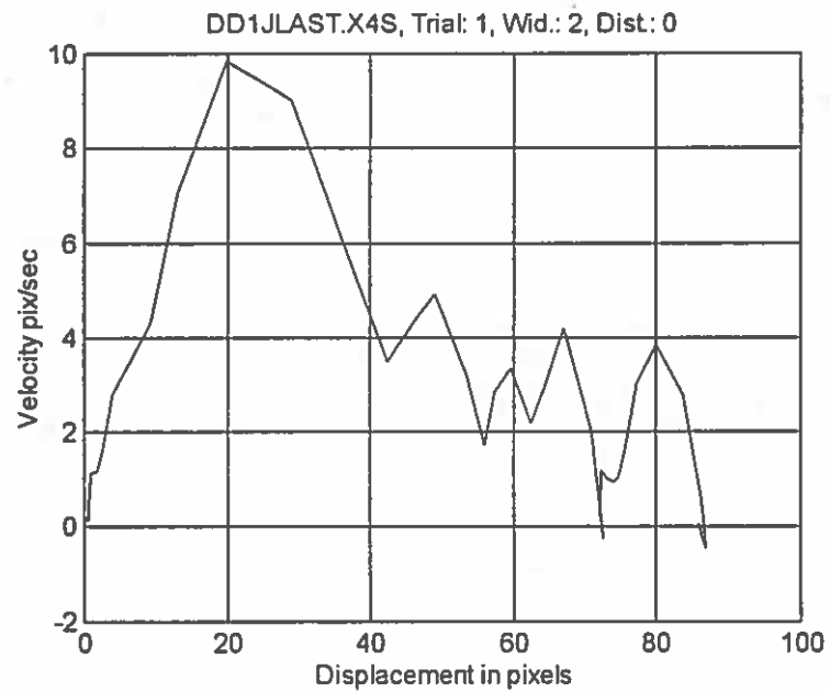
Figure 41. Last joystick trial by subject DD1 - Smoothed. A = 96 pixels.
