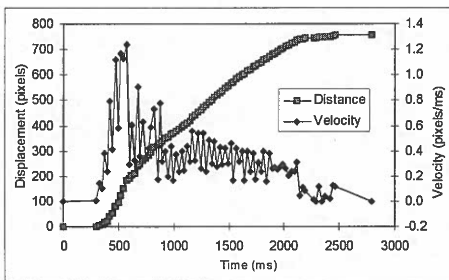
Figure 31. Isometric joystick - trial from preliminary tests. A = 768 pixels.
