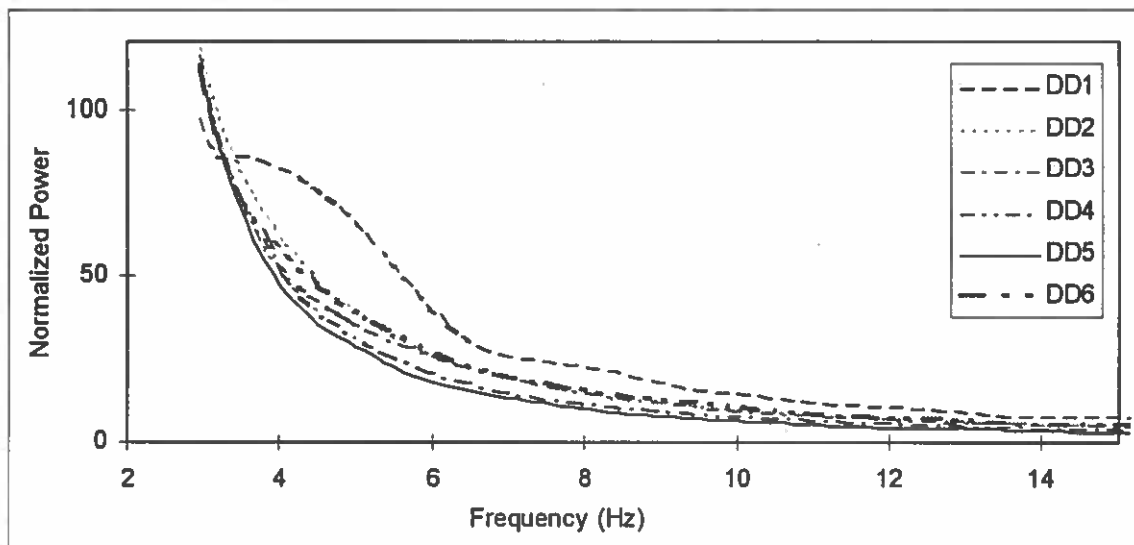
Figure 46. Spectrograms for last block of joystick trials.
