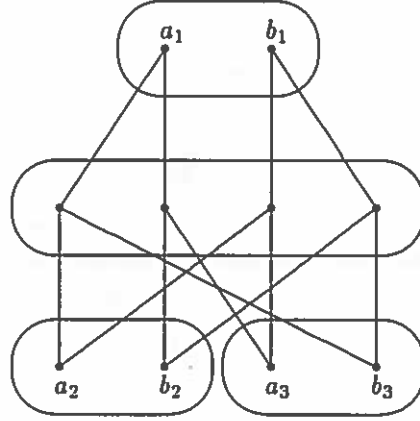
FIGURE 2. The graph \Xi_3
