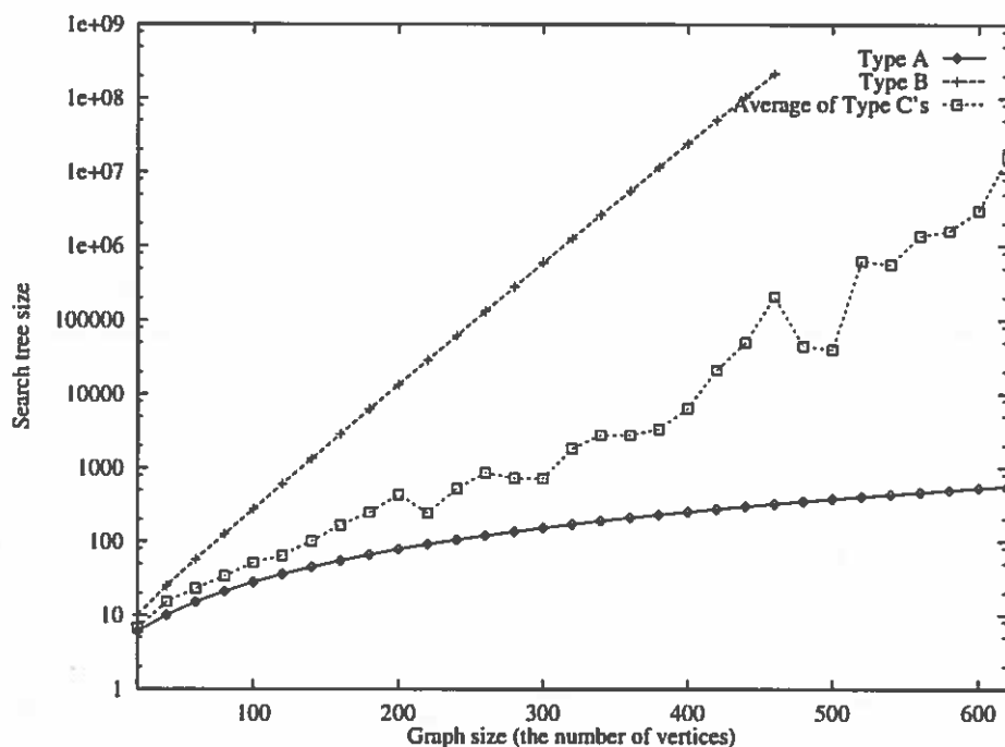
FIGURE 4. The number of tree nodes generated
