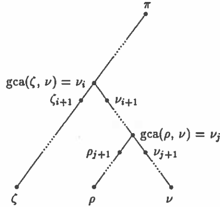
FIGURE 1. Pruning by automorphism equivalence
