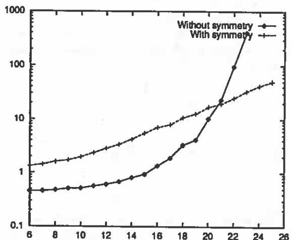
Figure 5: Average run times over 50 random perturbations with and without symmetry. Note that the y-axis is log scaled.
