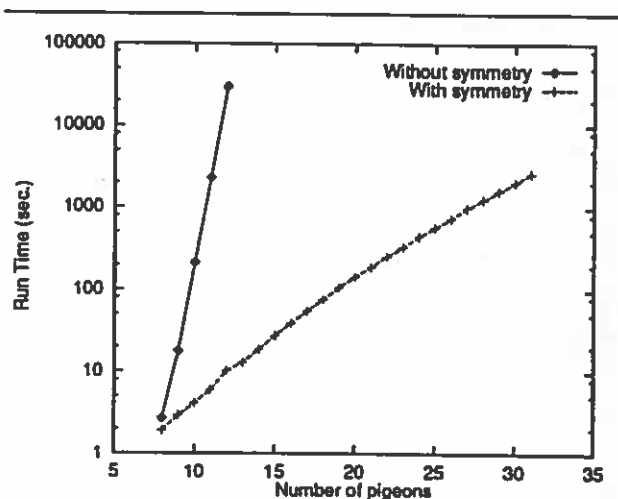
Figure 3: Run times for the pigeon-hole problem with and without symmetry. Note that the y axis is log scaled.
