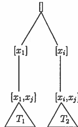
Figure 2: Symmetry trees for pruning example.
