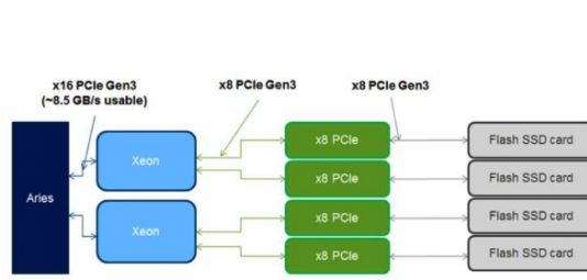
Figure 4: BurstBuffer node architecture. (Courtesy of NERSC.)
