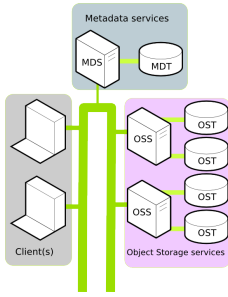
Figure 3: Lustre architecture. (Courtesy of Intel Wiki.)
